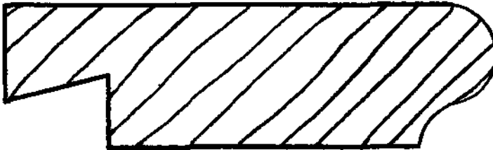
RB 9892-3 5 / 8 " RODENHAVEN WINDOW STOOL 1 1 / 16 " x 3 5 / 8 "
