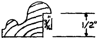
PARAN PANEL MOULD
