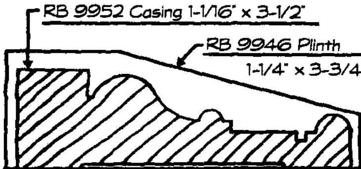
HARRIS RIDGE CASING
